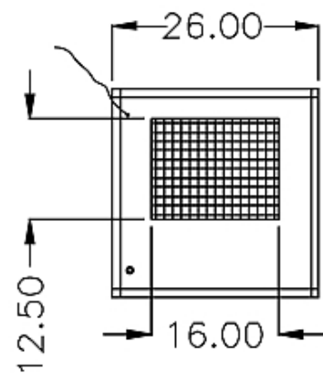
OUTLET VIEW
