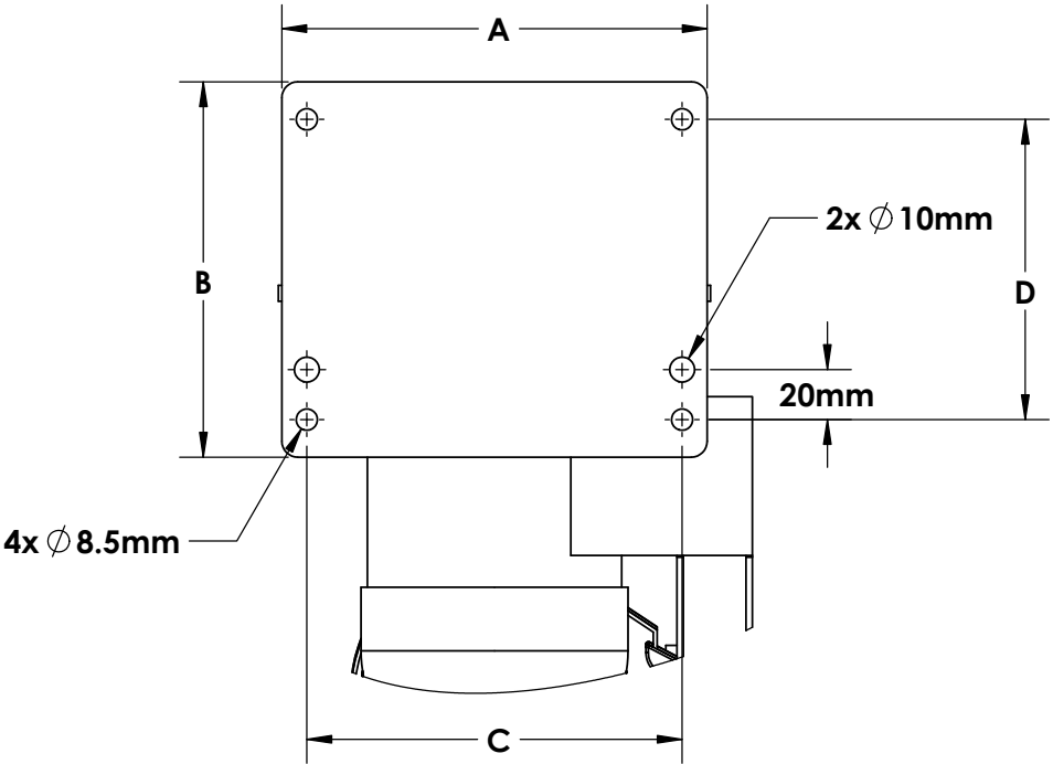
MOUNTING HOLE PATTERN
