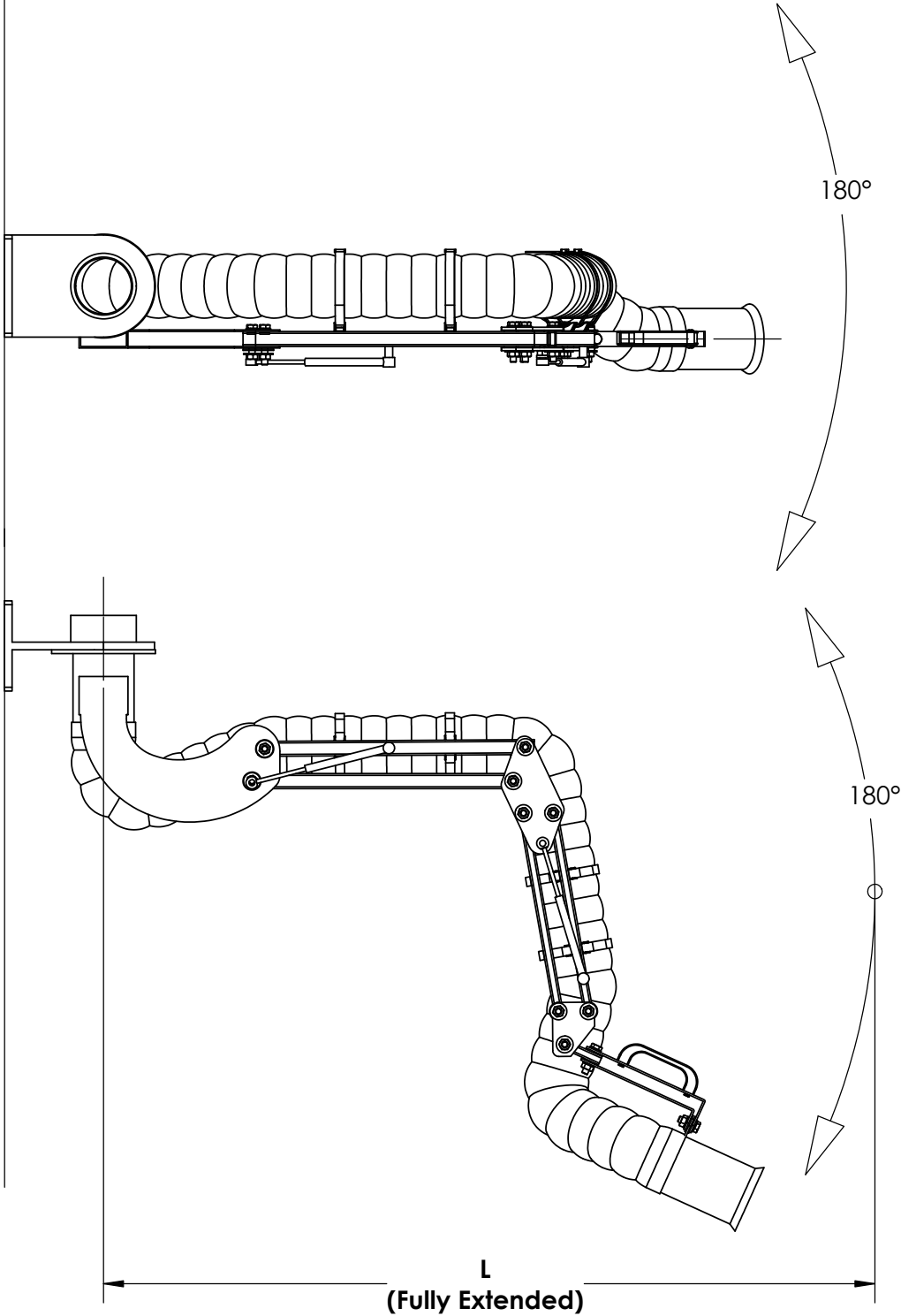
WALL / CEILING mounting
